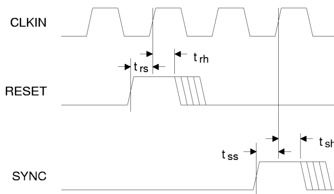
Figure 14. RESET Timing
