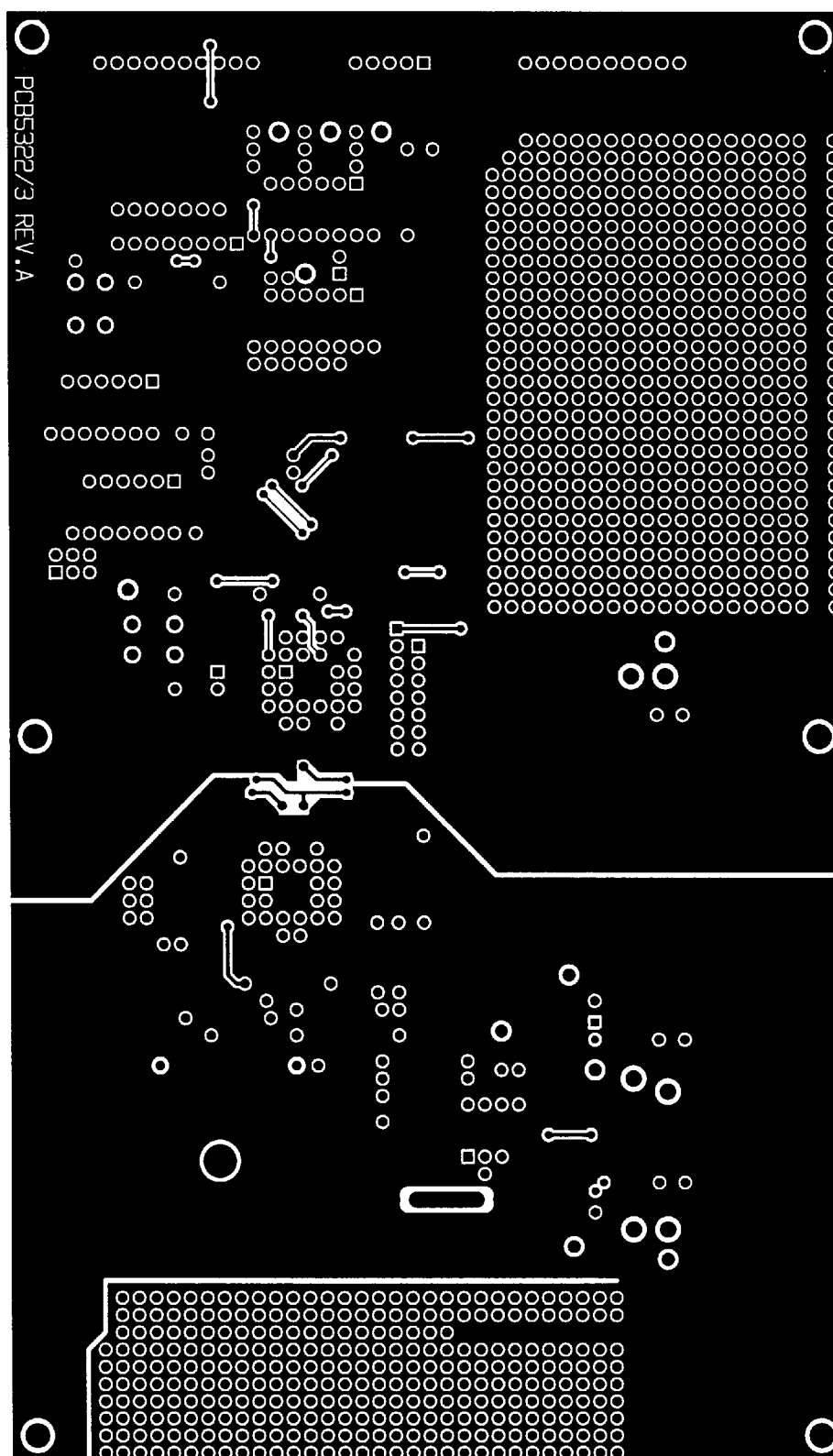
Figure 9. CDB5323 Ground Plane Layer (Not to Scale)
