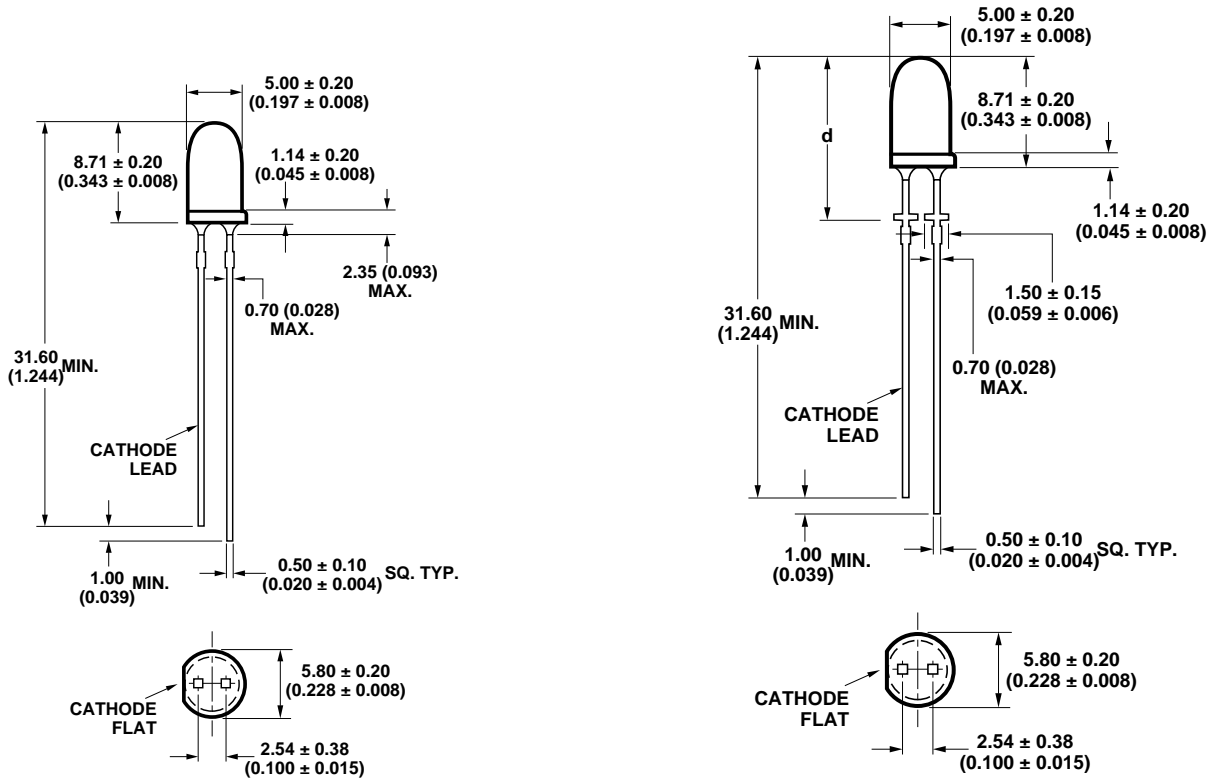
PACKAGE DIMENSION A
