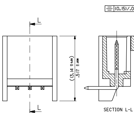
1 TO 6 CIRCUITS
