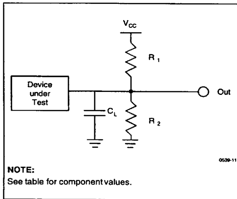
Figure 11. Test Configuration
