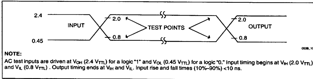
Figure 10. 5V Inputs and Measurement Points
