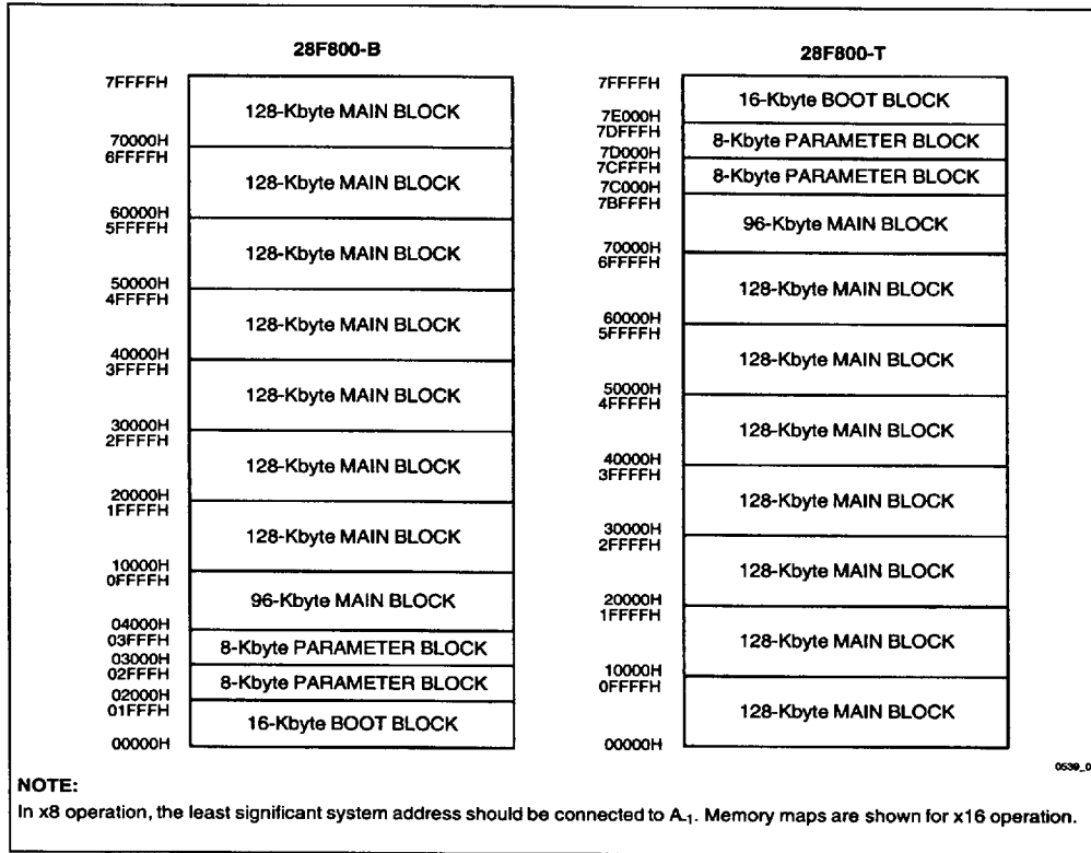
Figure 4. Word-Wide x16-Mode Memory Maps
