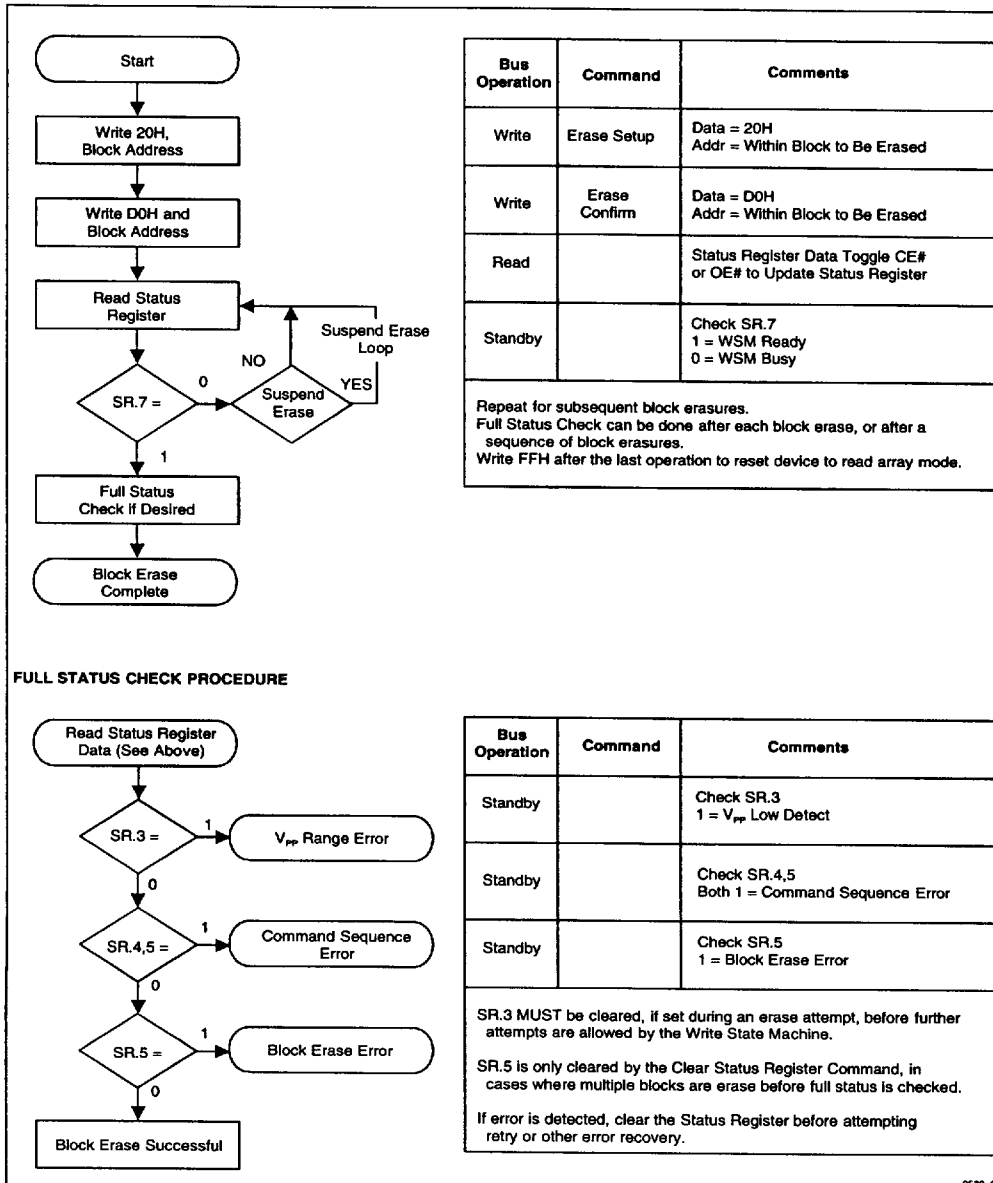
Figure 7. Automated Block Erase Flowchart
