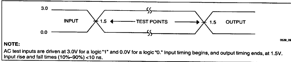
Figure 17. 3.3V Input Range and Measurement Points
