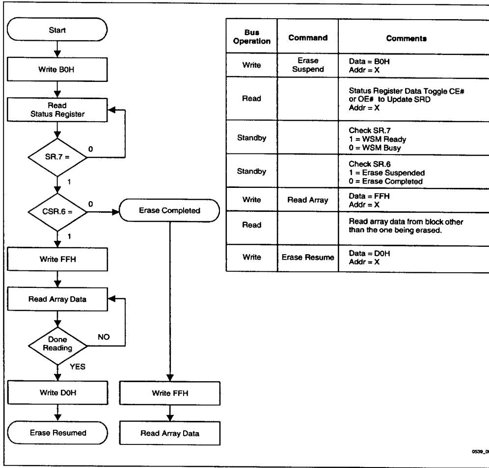
Figure 8. Erase Suspend/Resume Flowchart
