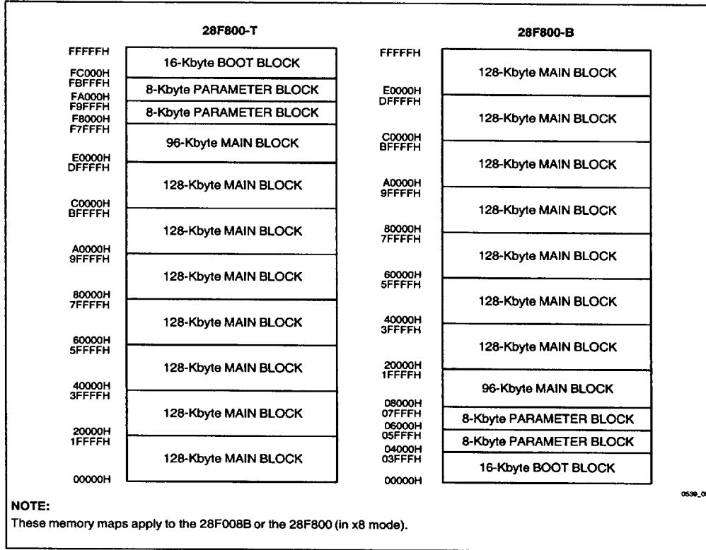
Figure 5. Byte-Wide x8-Mode Memory Maps
