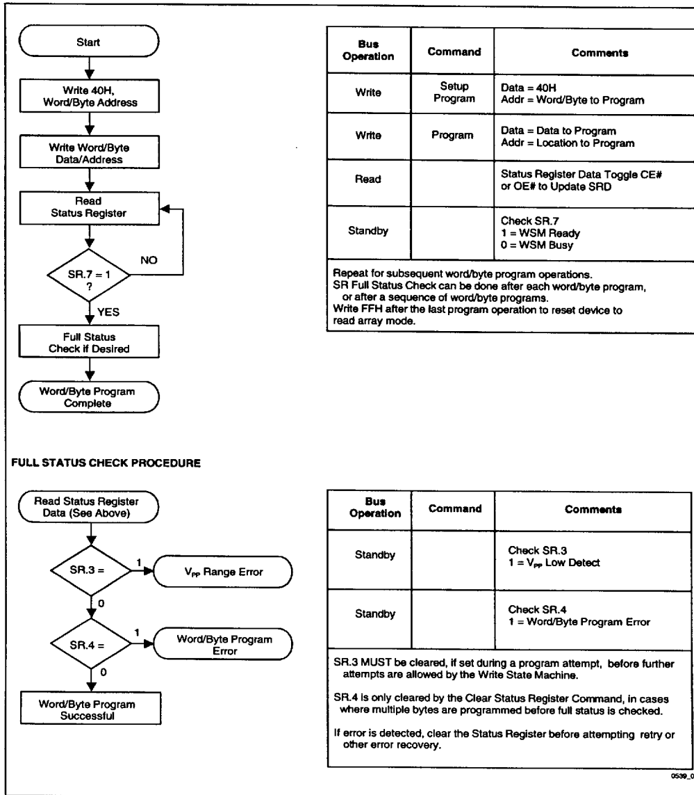
Figure 6. Automated Word/Byte Programming Flowchart
