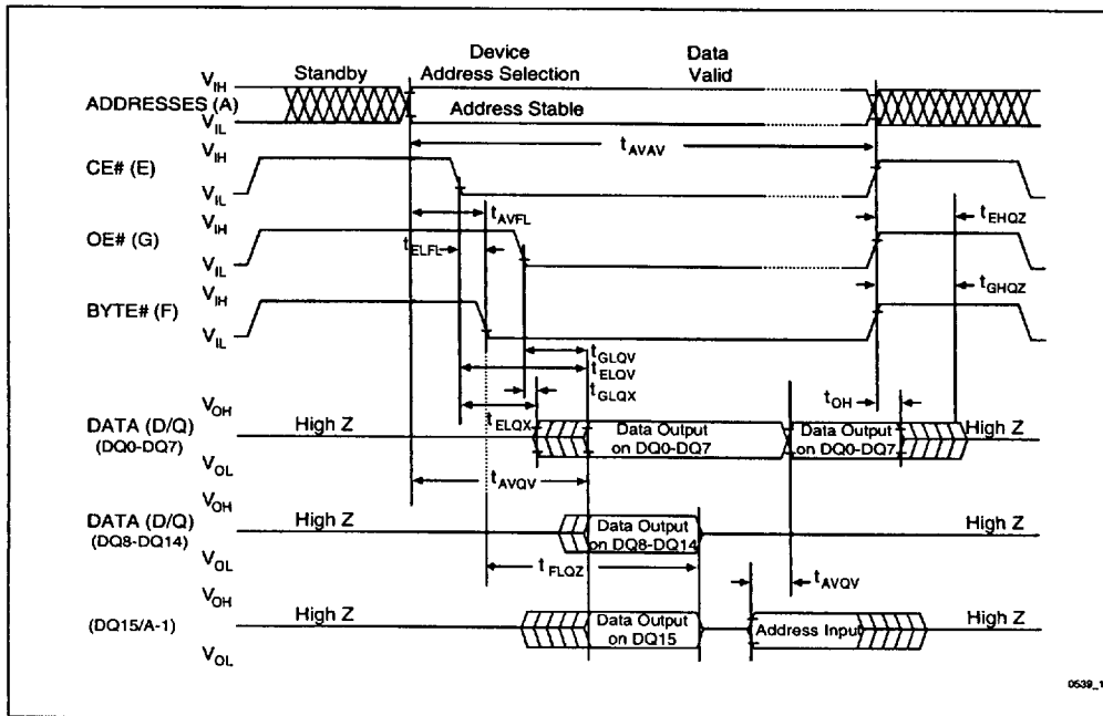
Figure 13. BYTE# Timing Diagram for Read Operations
