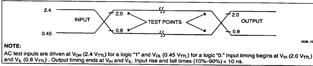
Figure 18. 5V Input Range and Measurement Points
