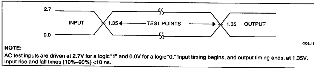
Figure 16. 2.7V–3.6V Input Range and Measurement Points
