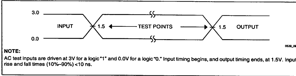
Figure 9. 3.3V Inputs and Measurement Points
