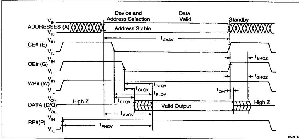
Figure 12. AC Waveforms for Read Operations
