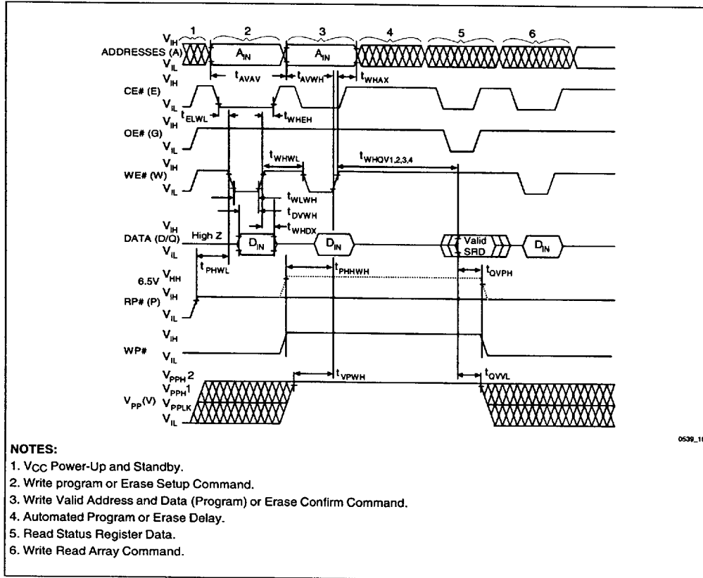
Figure 14. AC Waveforms for Write Operations (WE#-Controlled Writes)
