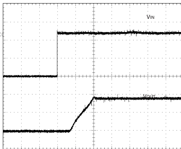
Typical Start-Up from VIN
