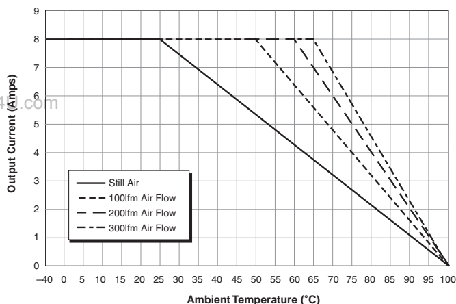
Temperature Derating for 8 Amp Models V IN = Nominal
