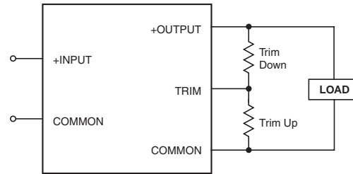
Figure 5. Trim Connections Using Fixed Resistors
