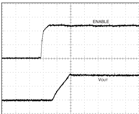
Typical Start-Up from Enable
