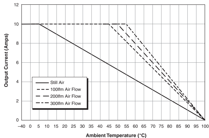
Temperature Derating for 10 Amp Models V IN = Nominal
