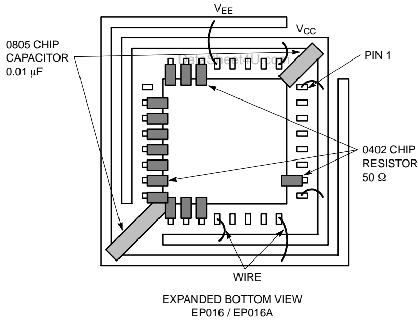
Figure 7. Configuration 2
