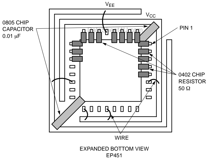
Figure 15. Configuration 10
