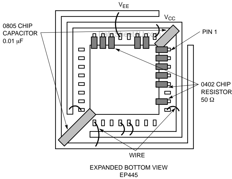
Figure 13. Configuration 8
