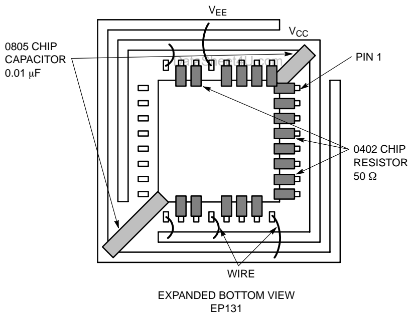
Figure 10. Configuration 5
