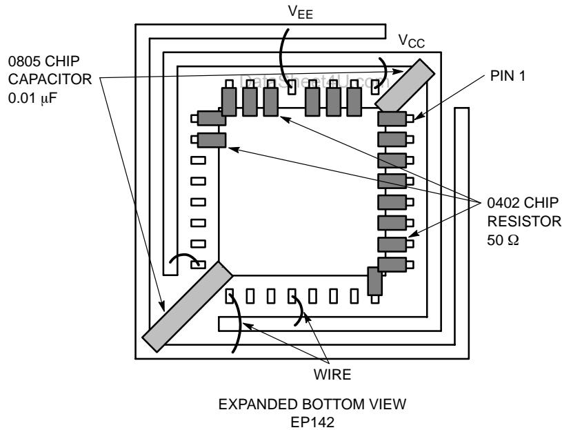
Figure 11. Configuration 6
