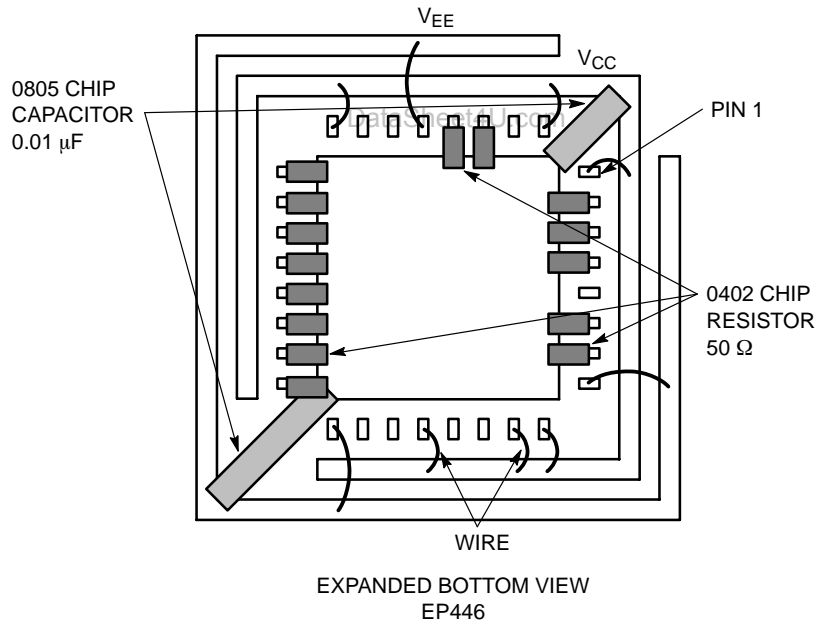
Figure 14. Configuration 9
