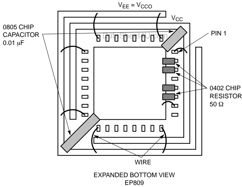
Figure 16. Configuration 11
