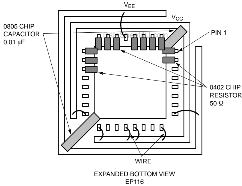
Figure 9. Configuration 4
