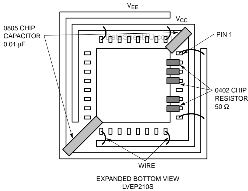
Figure 18. Configuration 13
