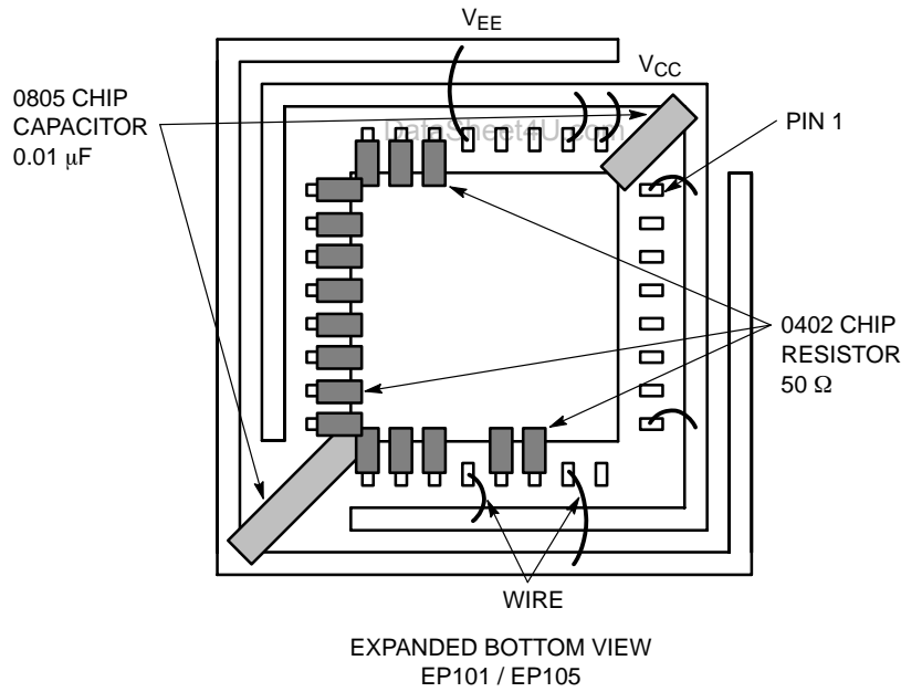
Figure 8. Configuration 3
