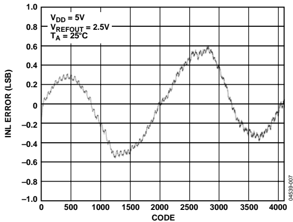
Figure 7. INL—AD5620-2/AD6520-3
