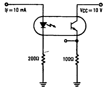
Test Circuit
