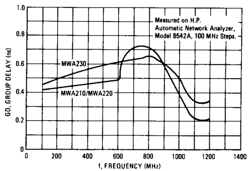
FIGURE 25 – GROUP DELAY versus FREQUENCY
