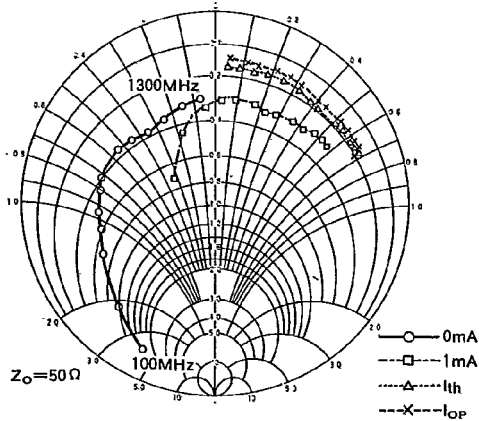
Fig. 12 Impedance characteristics
