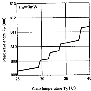
Fig. 6 Temperature dependence of peak wavelength
