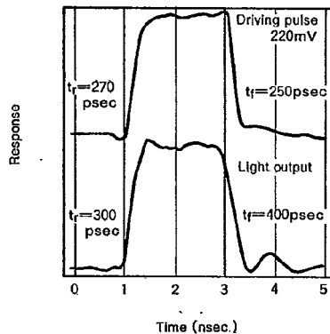
Fig. 9 Pulse response waveform
