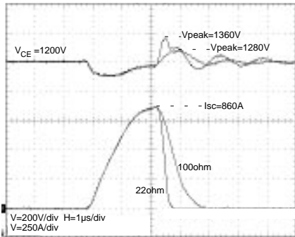
Fig.13 Effect of R_{goff-SC} in short - circuit
