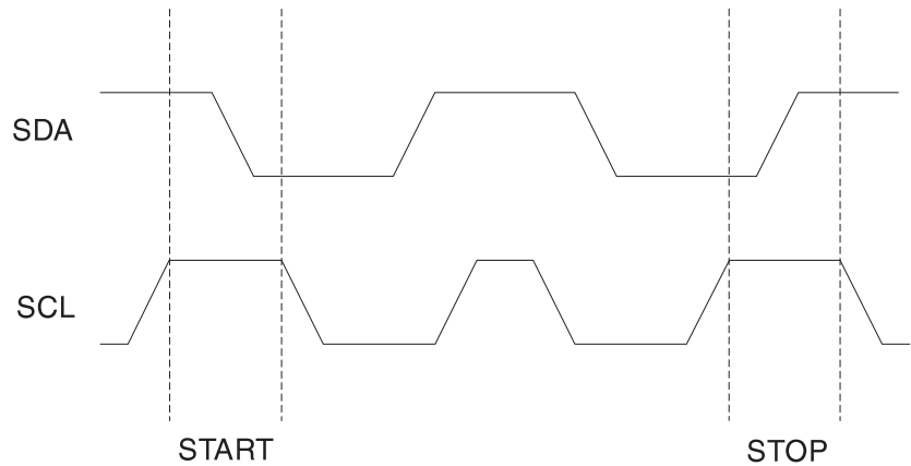
Figure 12. Start and Stop Definition
