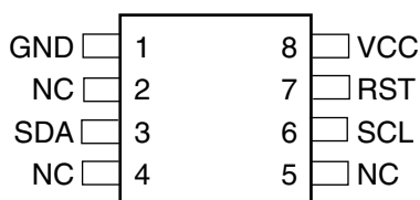
Figure 2. 8-pin SOIC, PDIP, or LAP
