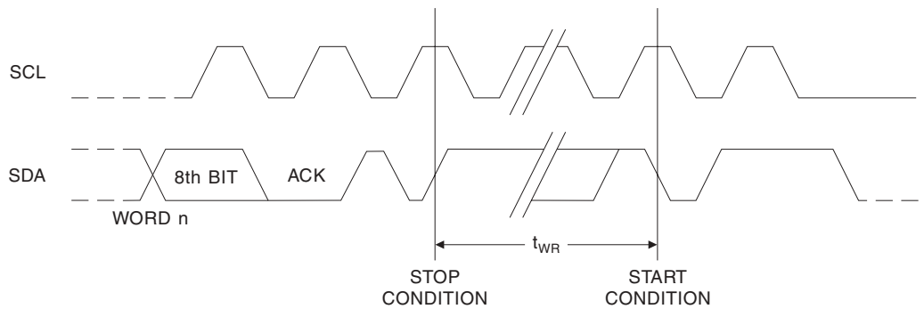
Figure 17. Write Cycle (SCL: Serial Clock; SDA: Serial Data I/O)
