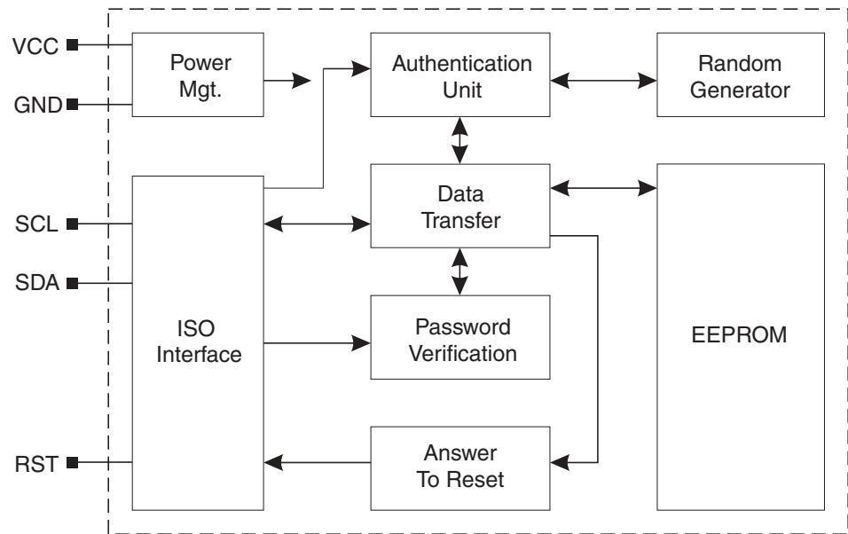
Figure 3. Block Diagram
