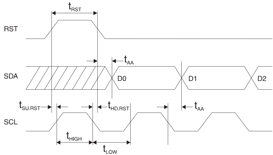
Figure 16. Synchronous Answer-to-reset Timing
