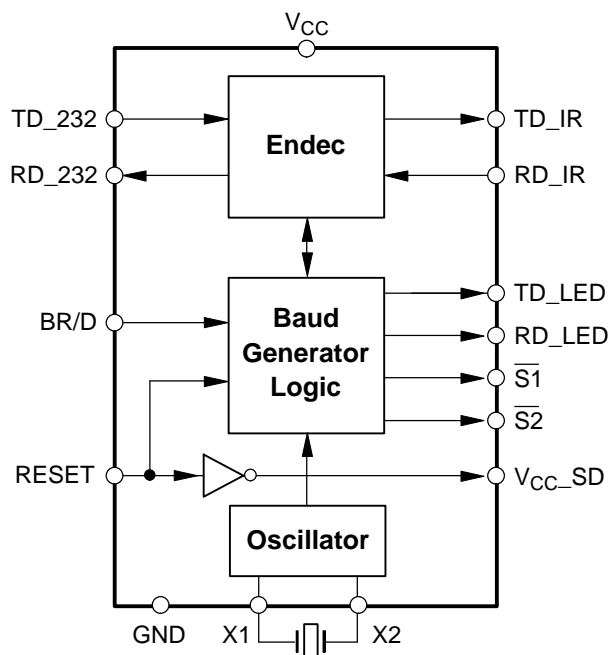
Figure 1. Block diagram
