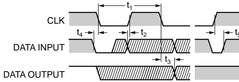
Serial Interface Timing
