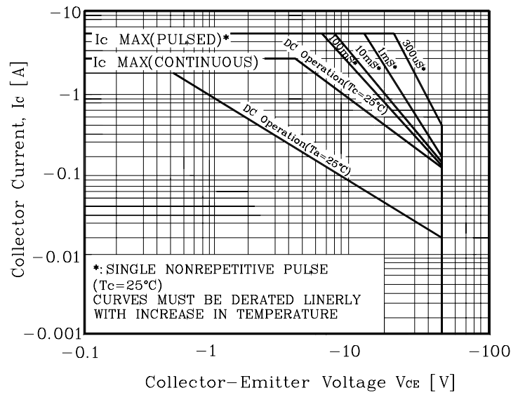
Fig. 8 Safe Operating Area
