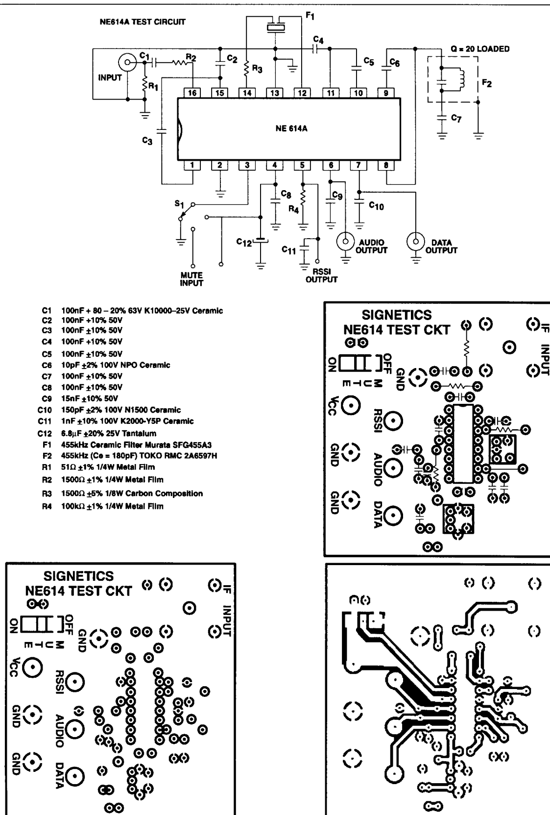
Figure 1. NE/SA614A Test Circuit
