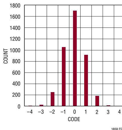
Figure 5. LTC1859 Histogram for 4096 Conversions
