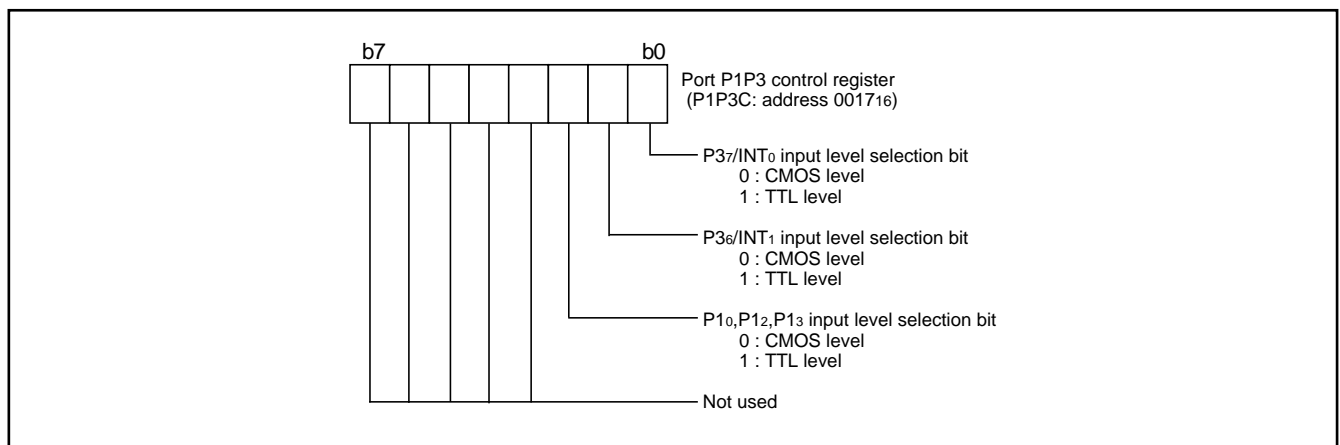
Fig. 10 Structure of port P1P3 control register
