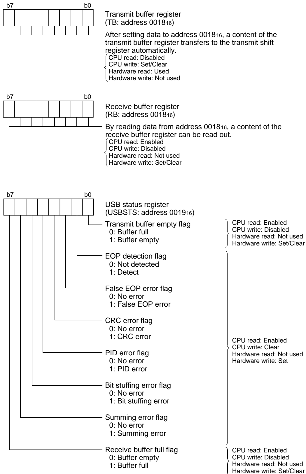
Fig. 24 Structure of serial I/O1-related registers (1)
