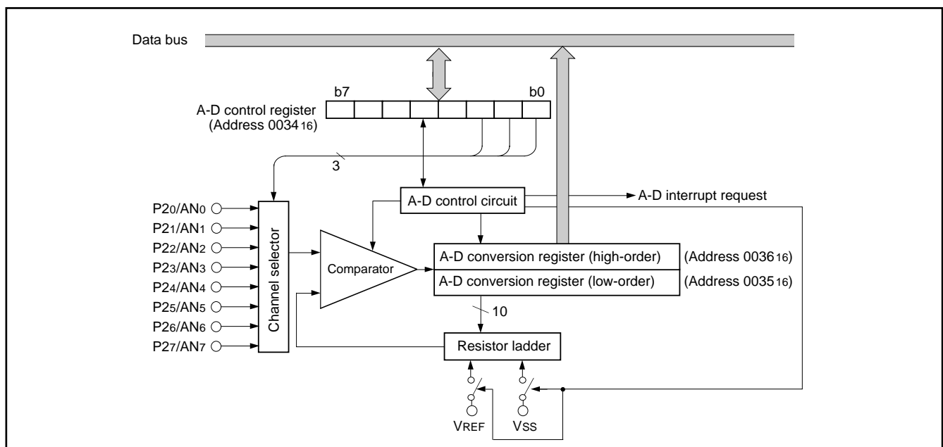
Fig. 34 Block diagram of A-D converter
