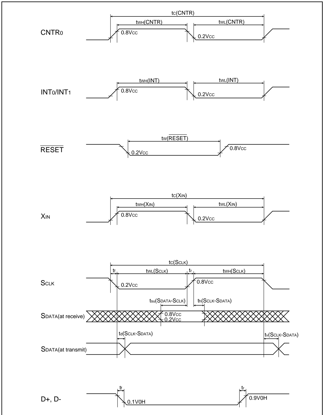
Fig. 47 Timing chart
