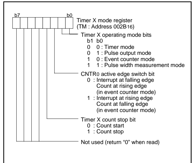
Fig. 16 Structure of timer X mode register
