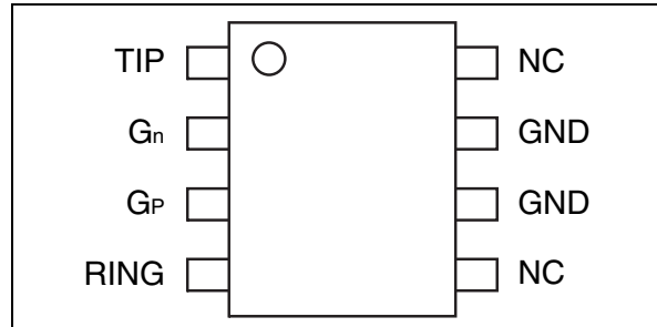
Figure 2. Pin-out configuration
