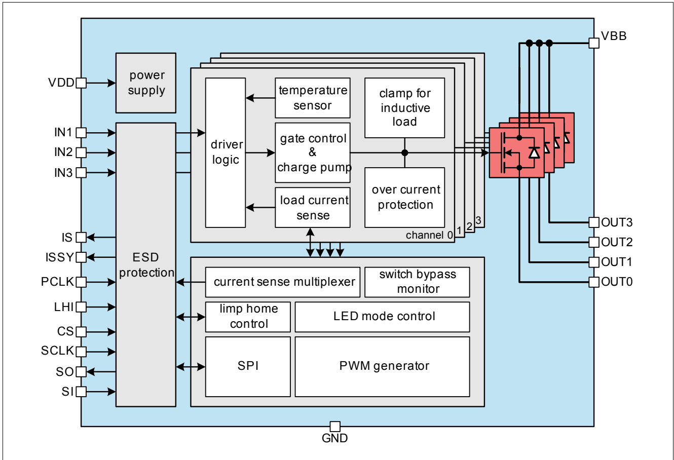
Figure 1 Block Diagram SPOC - BTS6460SF
