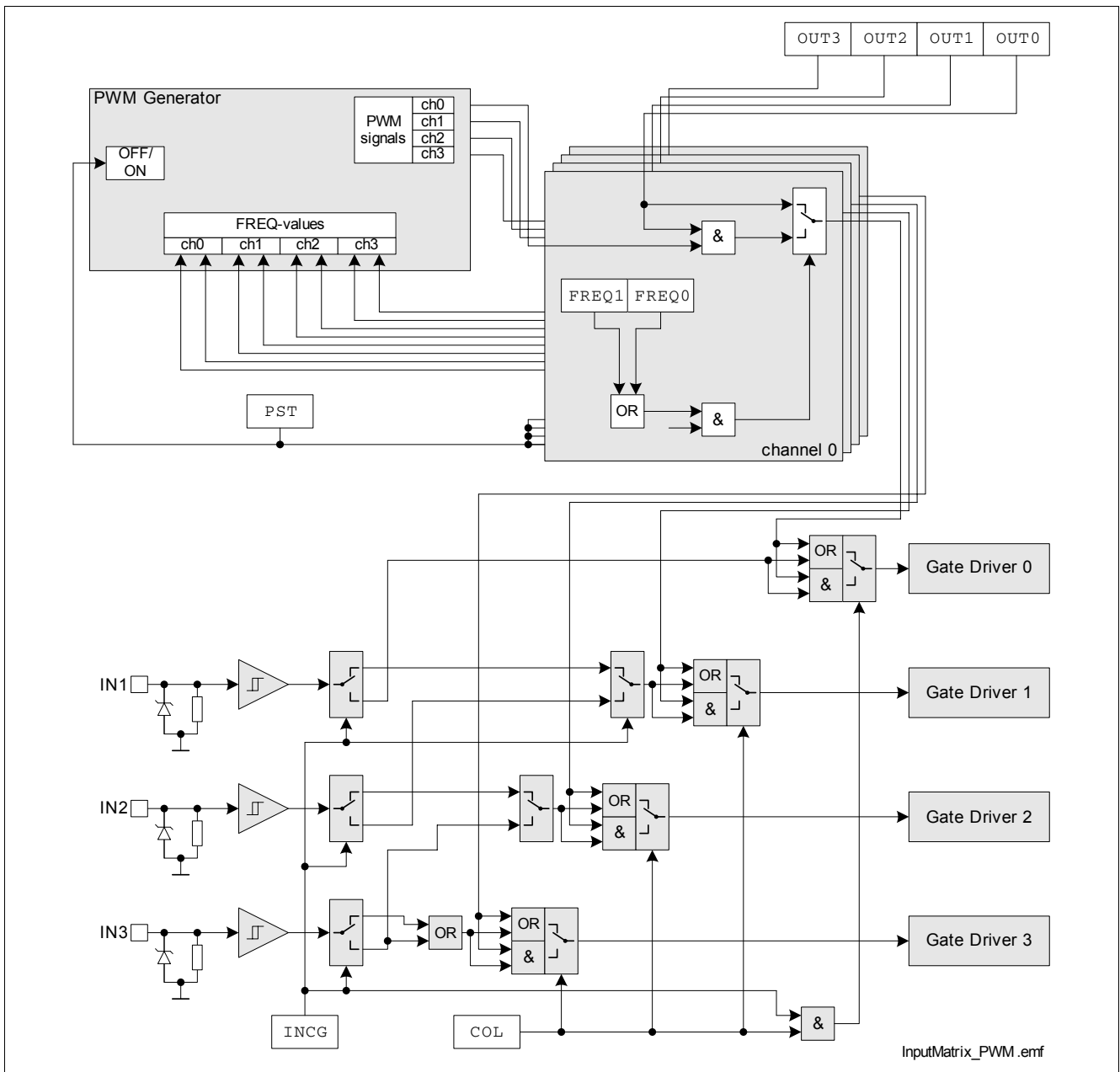
Figure 5 Input Switch Matrix
