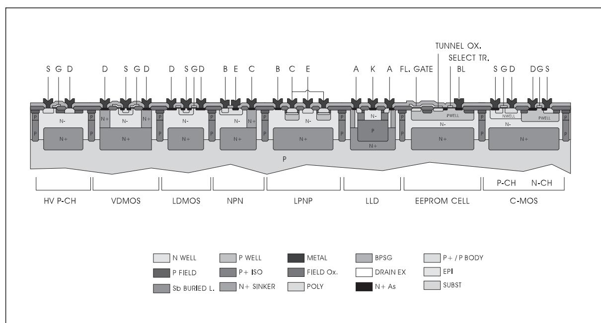
Figure 8: Multipower-BCD structure
