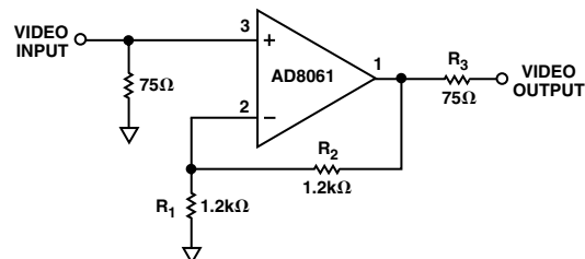
Figure 69. Recommended Output DAC Buffering
