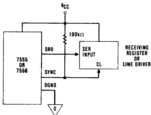
Figure 17. Serial Data Transfer
