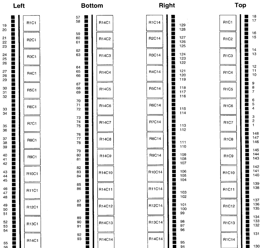
Figure 23: XC5206 CLB-to-Pad Relationship (Detail)
