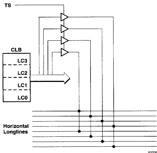
Figure 8: XC5200 3-State Buffer
