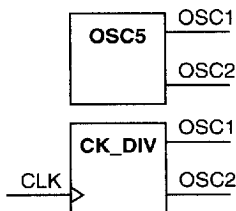
Figure 9: XC5200 Oscillator Macros
