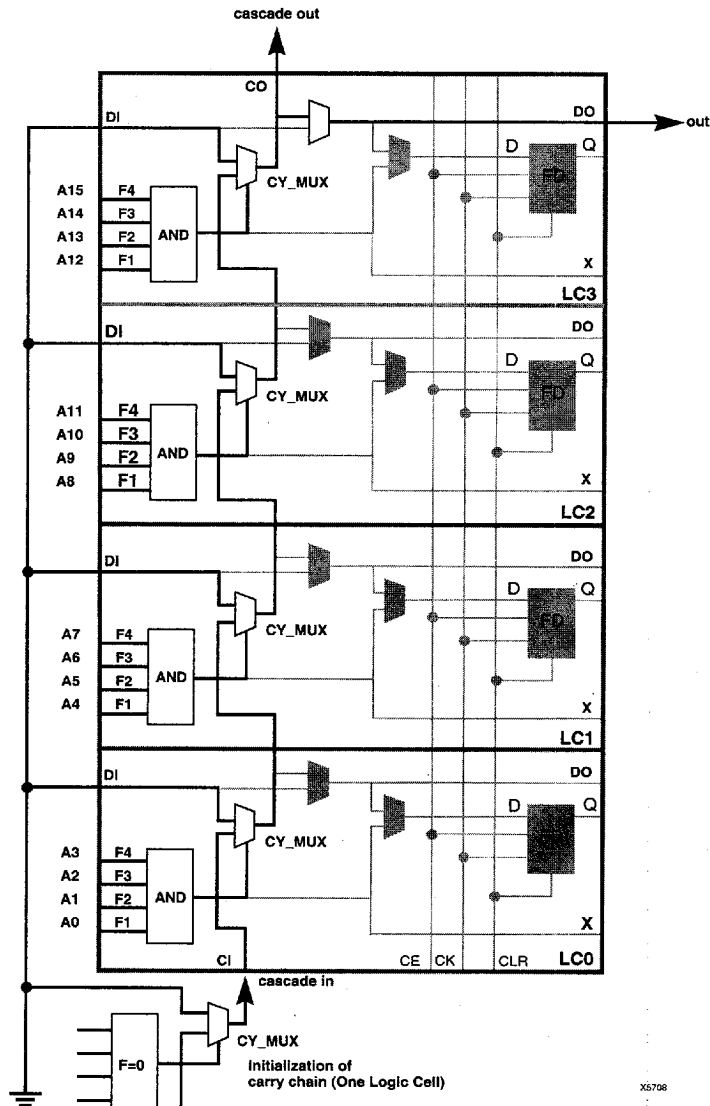
Figure 7: XC5200 CY_MUX Used for Decoder Cascade Logic
