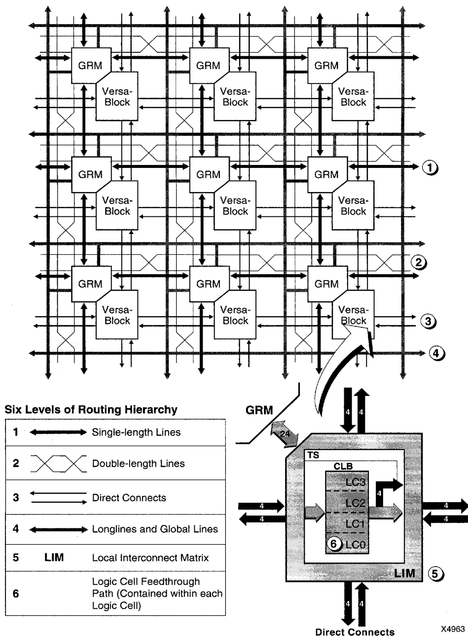
Figure 11: XC5200 Interconnect Structure
