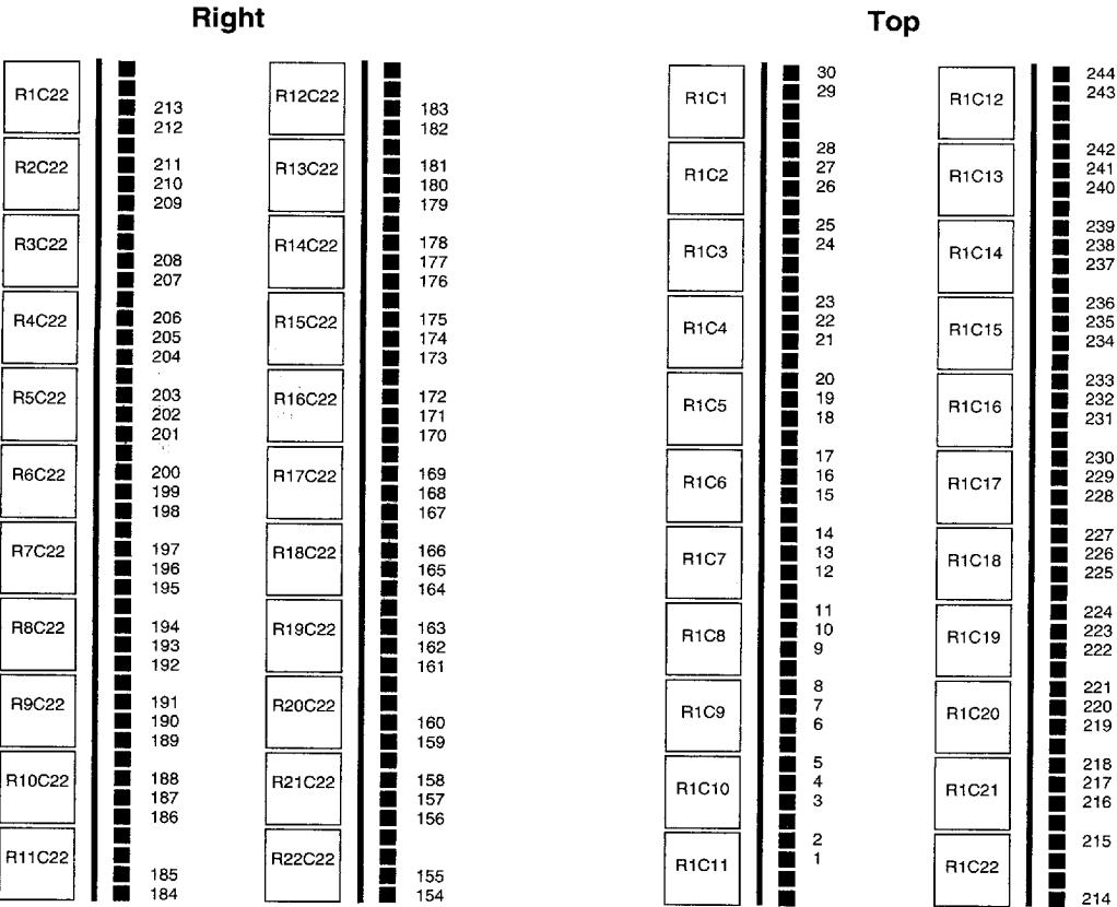
Figure 28: XC5215 CLB-to-Pad Relationship (Right/Top Detail)
