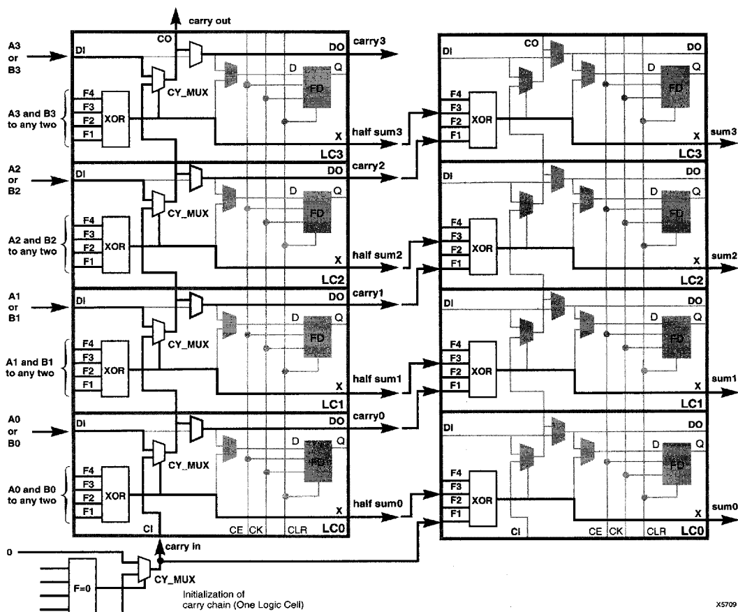
Figure 6: XC5200 CY_MUX Used for Adder Carry Propagate
