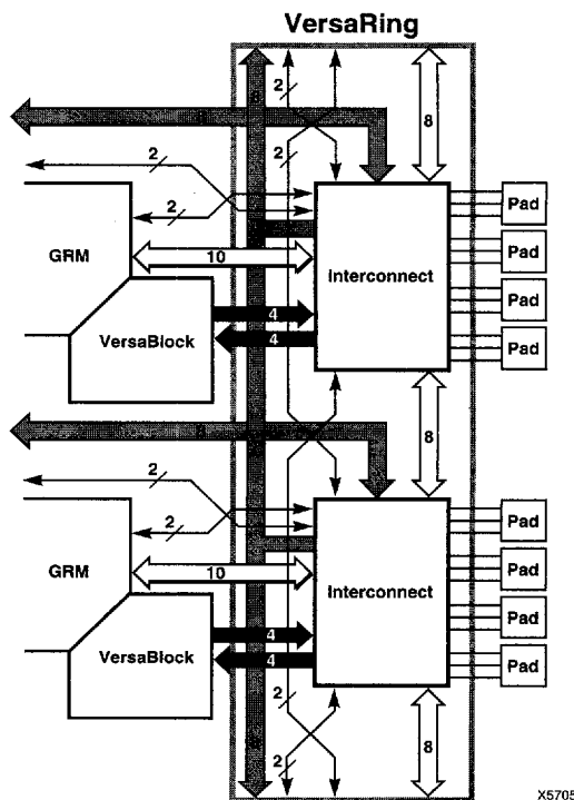
Figure 13: VersaRing I/O Interface
