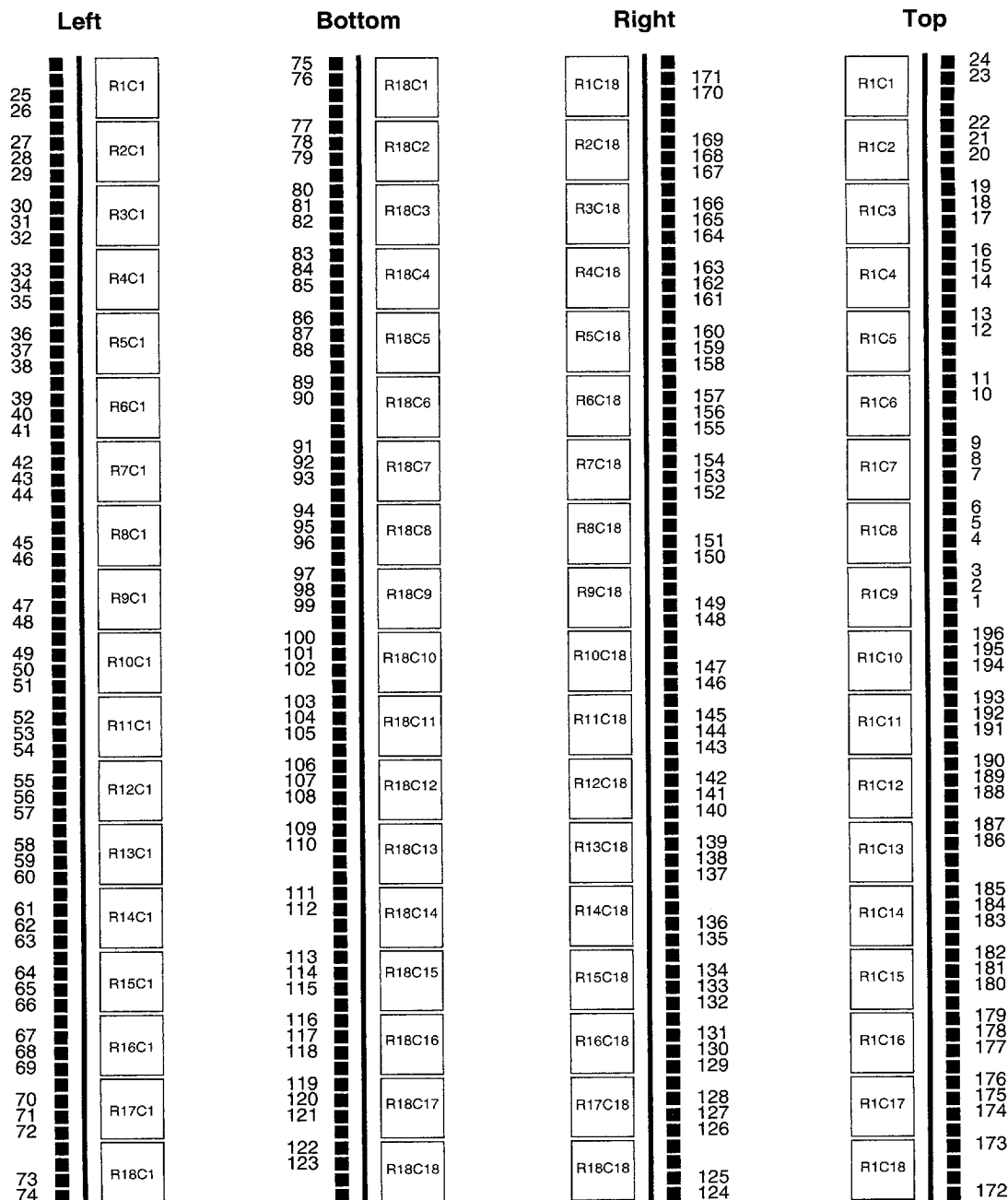
Figure 25: XC5210 CLB-to-Pad Relationship (Detail)
