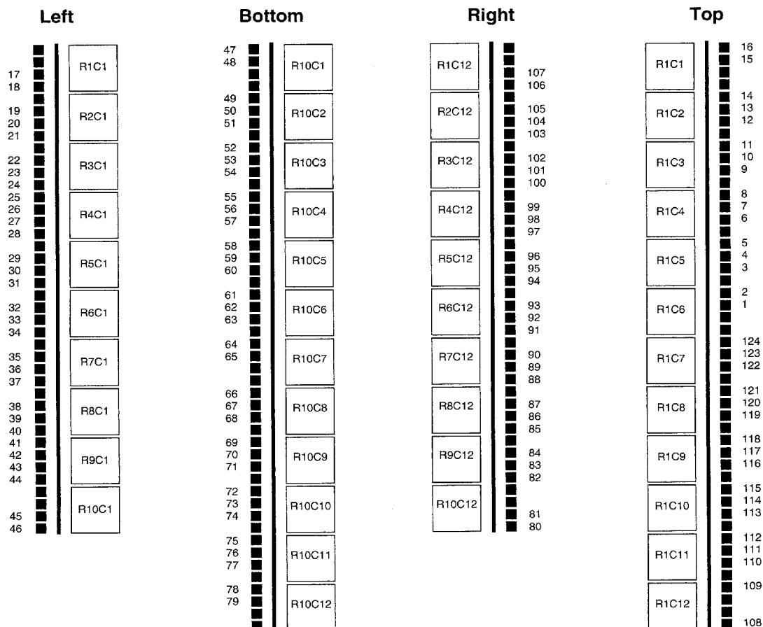
Figure 21: XC5204 CLB-to-Pad Relationship (Detail)
