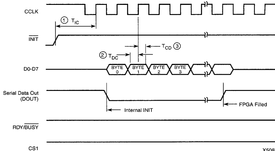
Figure 16: Express Mode Programming Switching Characteristics
