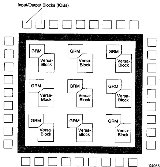
Figure 1: XC5200 Architectural Overview
