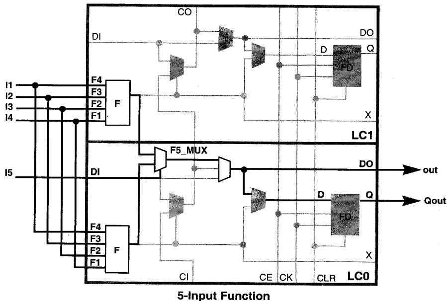
Figure 5: Two LUTs in Parallel Combined to Create a 5-input Function
