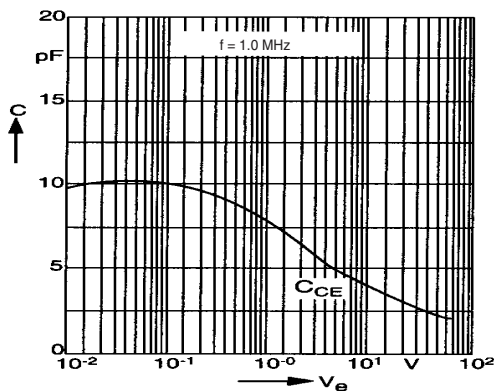
Figure 3. Transistor Capacitance (typ.) vs. Collector-Emitter Voltage
