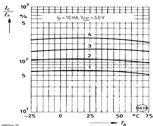
Figure 2. Current Transfer Ratio (typical) vs. Temperature
