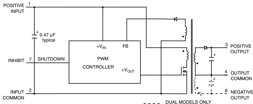
FIGURE 1: BLOCK DIAGRAM
