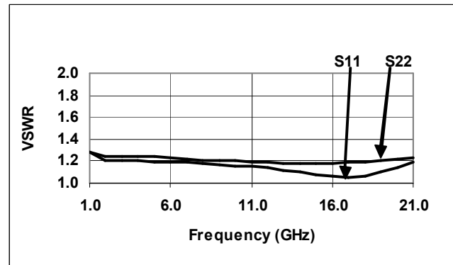
16 dB VSWR (S11, S22)
