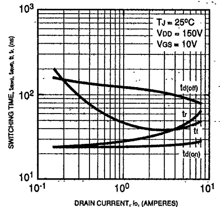
SWITCHING CHARACTERISTICS (TYPICAL) J934
