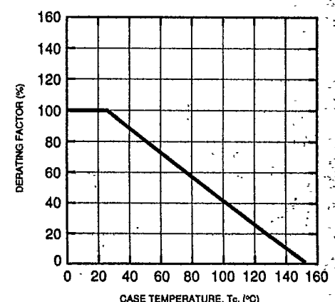
TEMPERATURE DERATING FACTOR OF SAFE OPERATING AREA (S.O.A.) J934
