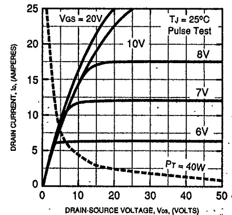
COMMON SOURCE OUTPUT CHARACTERISTICS (TYPICAL) J934
