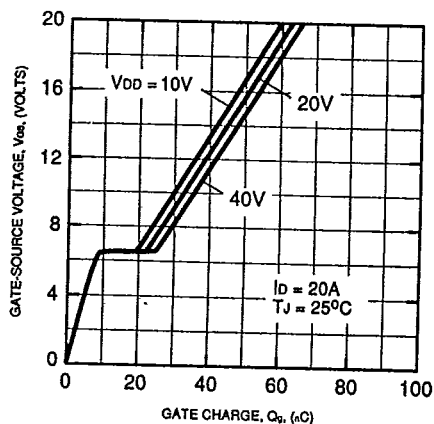
GATE CHARGE VS. V_{GS} (TYPICAL) J935
