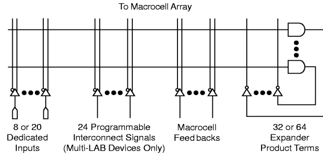
Figure 3. Expander Product Terms
