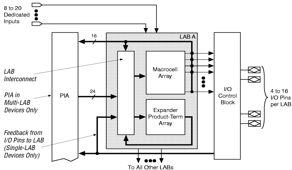
Figure 1. MAX 5000 Architecture
