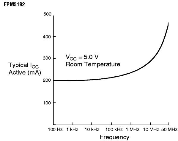
Figure 9. I_{CC} vs. Frequency for MAX 5000 Devices (Part 2 of 2)
