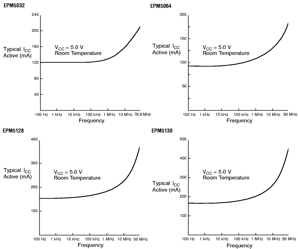
Figure 9. I_{CC} vs. Frequency for MAX 5000 Devices (Part 1 of 2)
