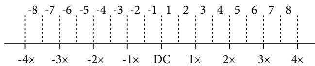
Figure 39. Nyquist Zones
