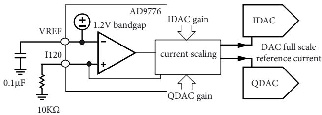
Figure 29. Reference Circuitry
