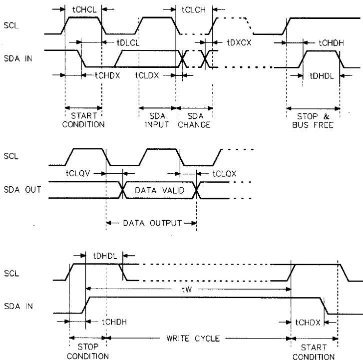
Figure 6. AC Waveforms
