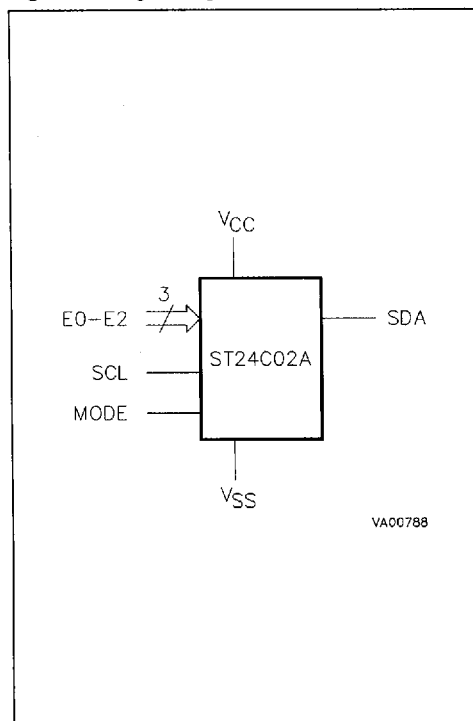
Figure 1. Logic Diagram
