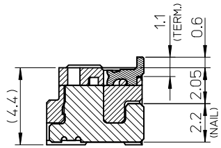
SECTION Z-Z
