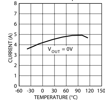
MIC29300-5.0 Short Circuit Current vs. Temperature
