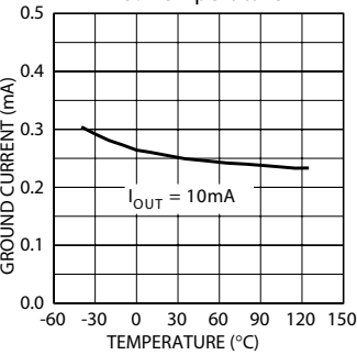
MIC2930x Ground Current vs. Temperature
