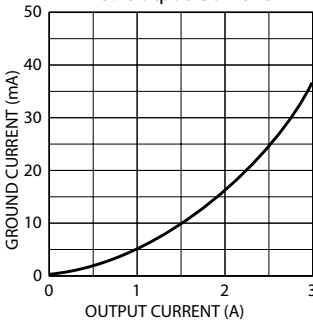
MIC2930x Ground Current vs. Output Current
