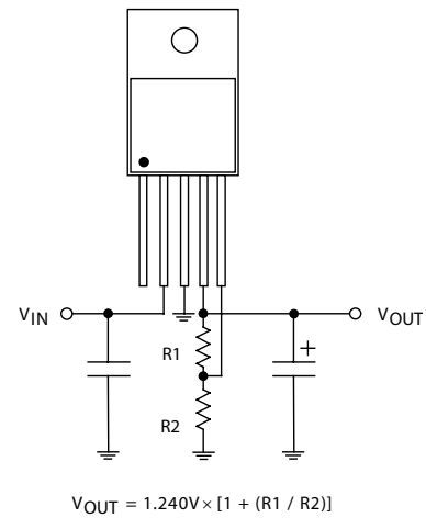
Figure 1. Adjustable output Voltage Configuration. For best results, the total series resistance should be small enough to pass the minimum regulator load current.
