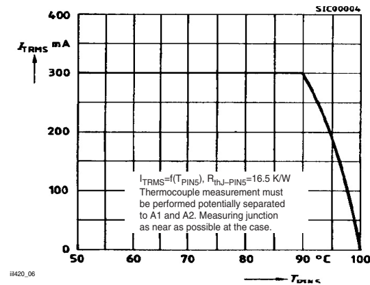
Figure 6. Current Reduction
