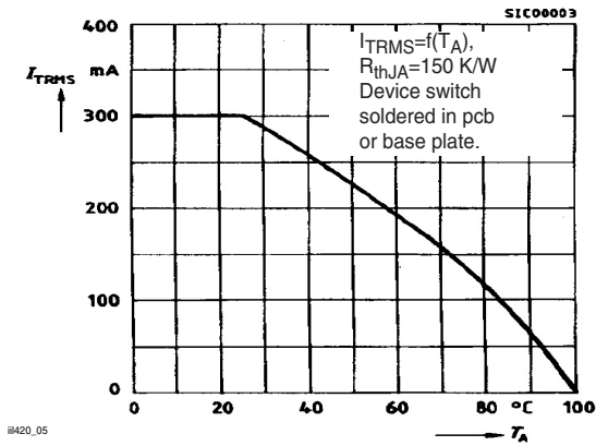
Figure 5. Current Reduction
