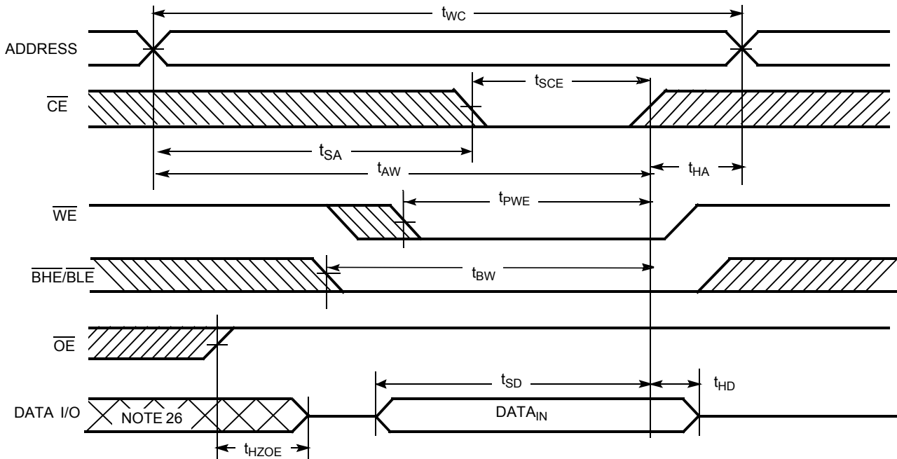
Figure 5. Write Cycle No. 2: \overline{\text{CE}} Controlled [23, 24, 25]
