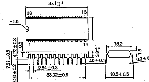
DIP 28pin
