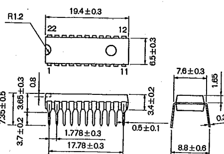
SDIP 22pin
