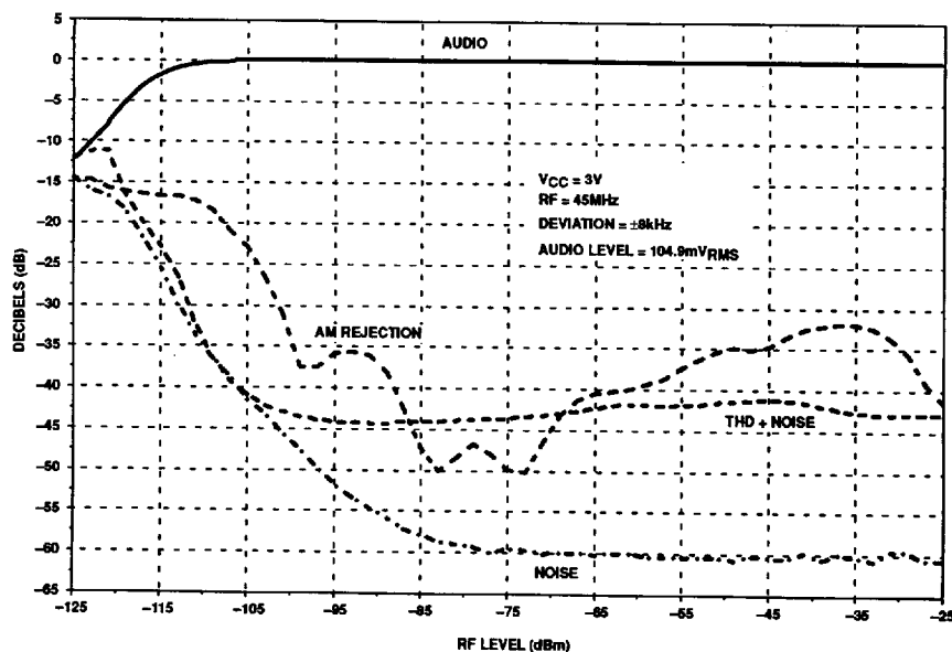
Figure 9. Sensitivity vs RF Level (-40°C)
