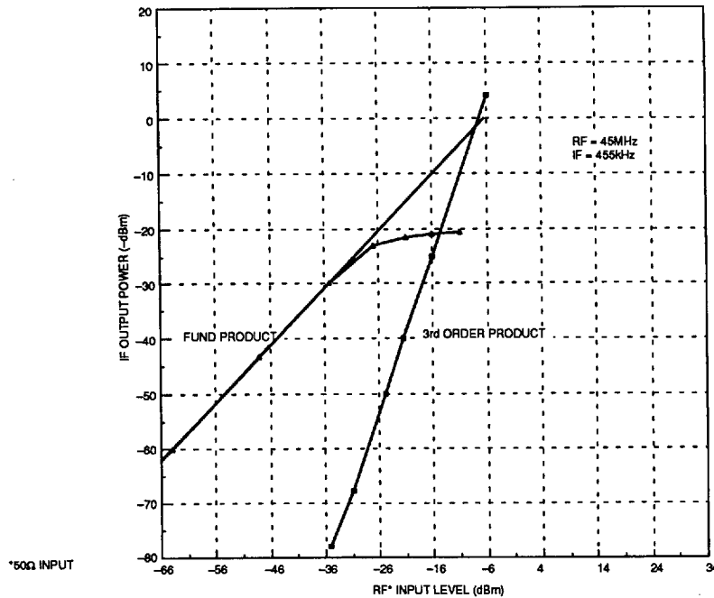
Figure 8. Mixer Third Order Intercept and Compression
