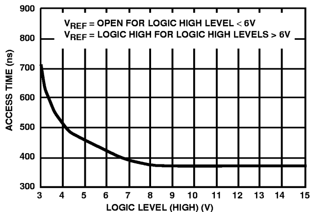
FIGURE 6A. ACCESS TIME vs LOGIC LEVEL (HIGH)
