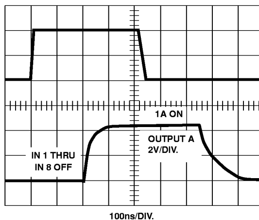
FIGURE 9C. ENABLE DELAY WAVEFORMS
