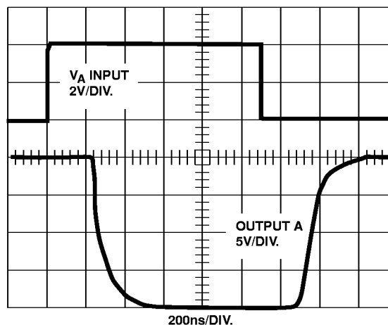
FIGURE 7B. ACCESS TIME WAVEFORMS
