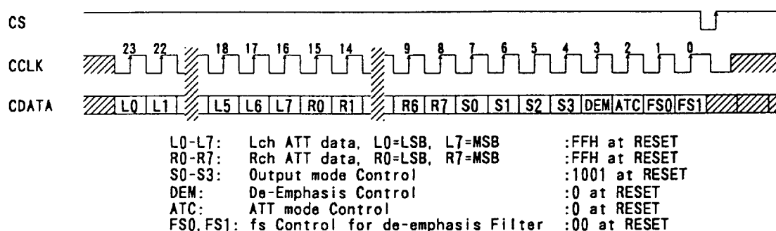
Figure 6. Serial mode control timing
