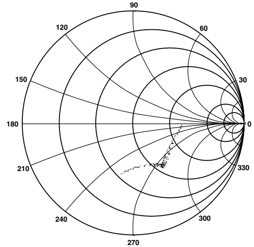
TPC 28. Input Impedance, Z_O = 50 \Omega , Differential Drive
