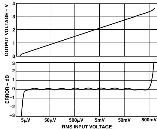
Figure 25. Output and Conformance for the AD8330/AD8362 Collaboration
