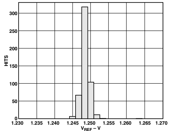
TPC 30. V_{REF} Distribution
