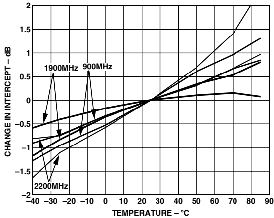
TPC 20. Change in Logarithmic Intercept vs. Temperature, 3 Sigma to Either Side of Mean, Frequencies 900 MHz, 1900 MHz, and 2200 MHz
