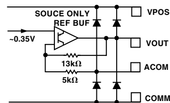
Circuit E
