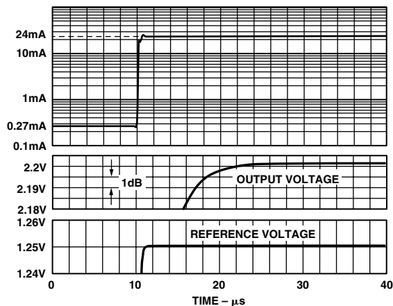
Figure 10. Typical “Wake-up” Response; t_0 = 10 \mu s
