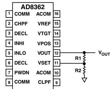
Figure 19. External Network to Raise Slope
