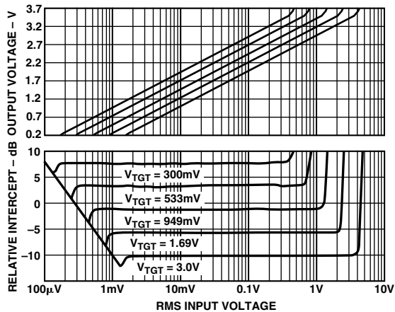
Figure 8. Response with V_{TGT} Varied from 0.3 V to 3 V in 5 dB Steps, Showing the Proportional Shift in Intercept
