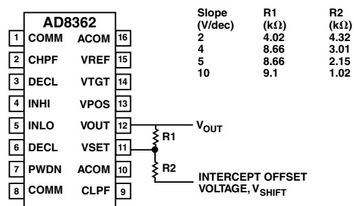
Figure 28. Slope and Intercept Adjustment
