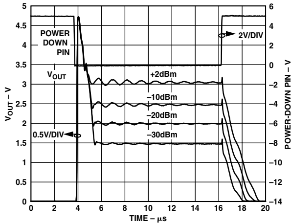
TPC 25. Output Response Using Power-Down Mode for Various RF Input Levels, Carrier Frequency 900 MHz, C_{LPF} = 0
