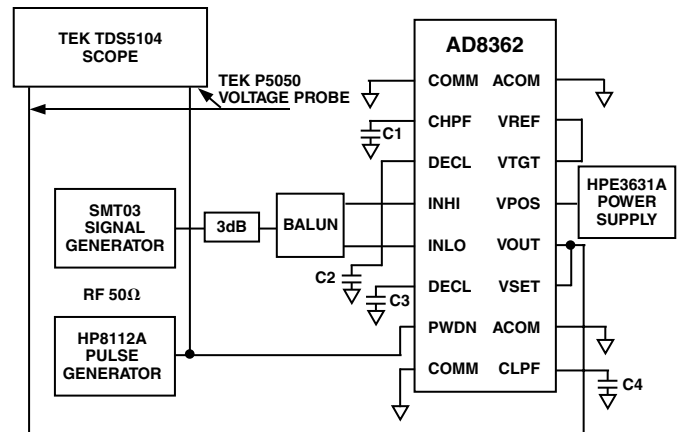
Figure 3. Response Measurement Setup for Power-Down Step
