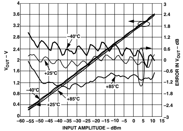
TPC 5. V_{OUT} and Law Conformance vs. Input Amplitude, Frequency 2200 MHz, Sine Wave, Temperature -40^{\circ}\text{C} , +25^{\circ}\text{C} , and +85^{\circ}\text{C}
