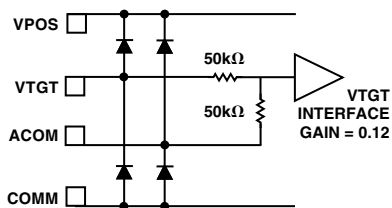
Circuit D
