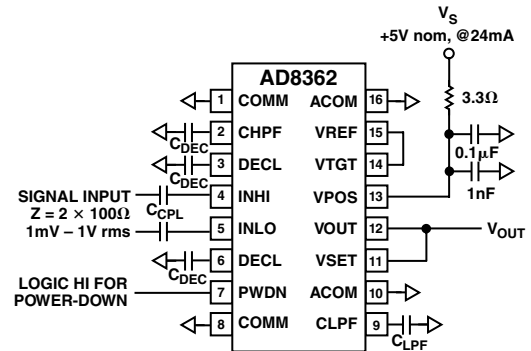
Figure 11. Basic Measurement Mode Connections
