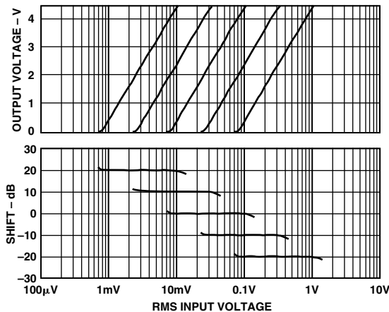
Figure 30. Illustrative Results for Slope of 200 mV/dB
