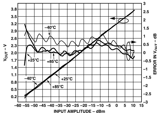
Figure 14. Output Voltage and Law Conformance Error, at T_A = -40^\circ\text{C} , +25^\circ\text{C} and +85^\circ\text{C}
