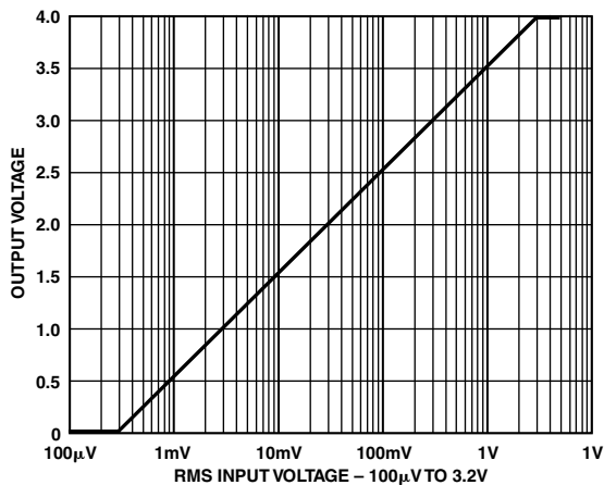
Figure 6. Ideal Response of the AD8362
