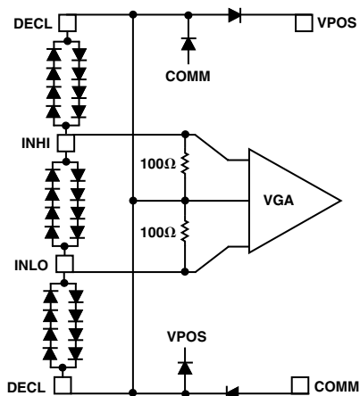
Circuit A
