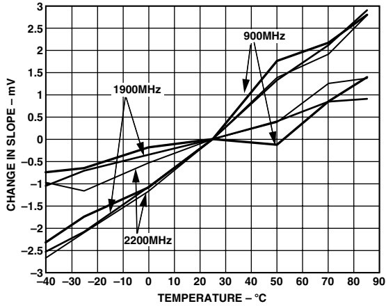
TPC 19. Change in Logarithmic Slope vs. Temperature, 3 Sigma to Either Side of Mean, Frequencies 900 MHz, 1900 MHz, 2200 MHz
