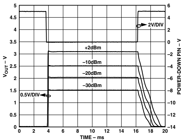
TPC 26. Output Response Using Power-Down Mode for Various RF Input Levels, Carrier Frequency 900 MHz, C_{LPF} = 0.1 \mu F
