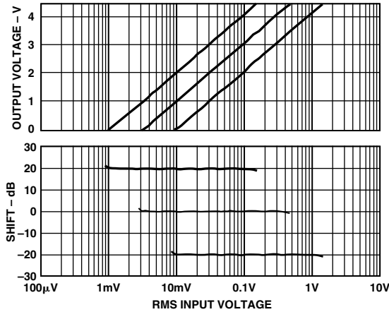
Figure 29. Illustrative Results for Slope of 100 mV/dB
