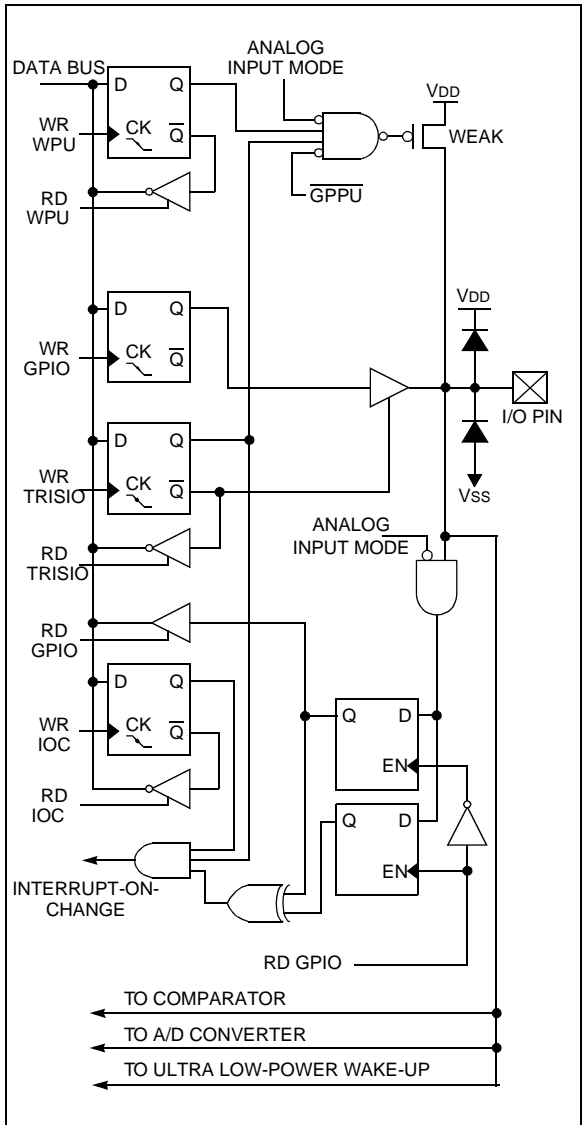
FIGURE 4-2: BLOCK DIAGRAM OF GP0
