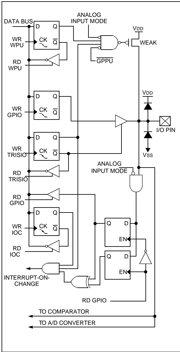
FIGURE 4-3: BLOCK DIAGRAM OF GP1
