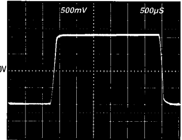
MAX406 (DECOMPENSATED MODE) LARGE-SIGNAL TRANSIENT RESPONSE
