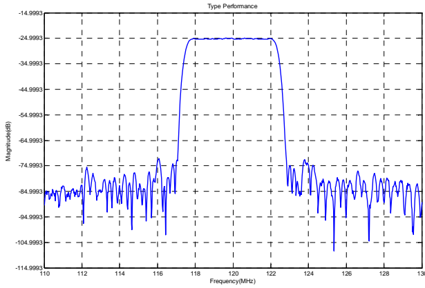
Frequency Respond
