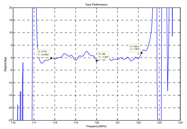
Phase Linearity(f0±2.2MHz)
