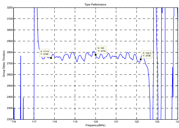
Group Delay Variation(f0±2.2MHz)
