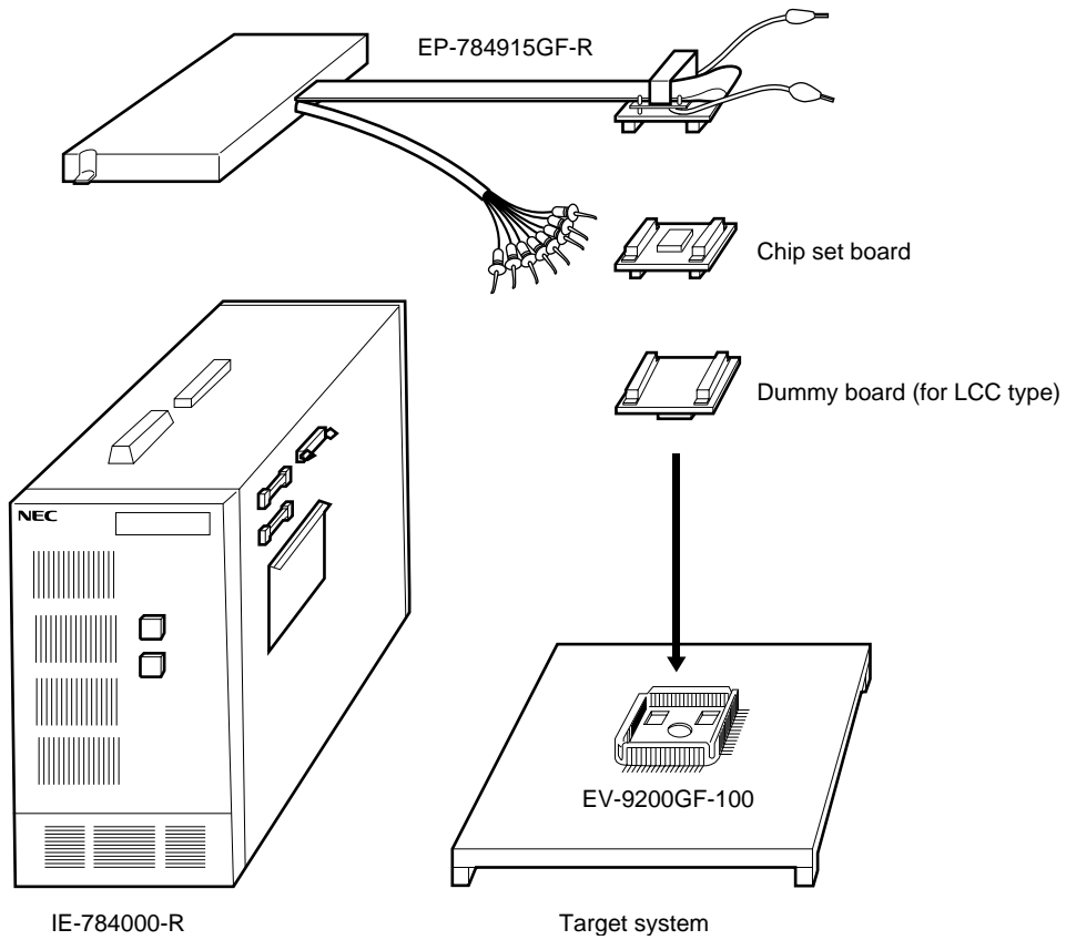
Figure 2-2. Example of Connection of EP-784915GF-R and Target System (LCC Type)
