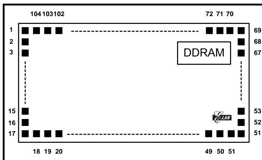
Figure 1 Pin Configuration
