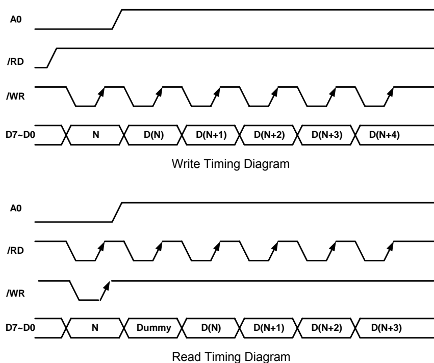
Figure 5 Write and Read Timing Diagrams
