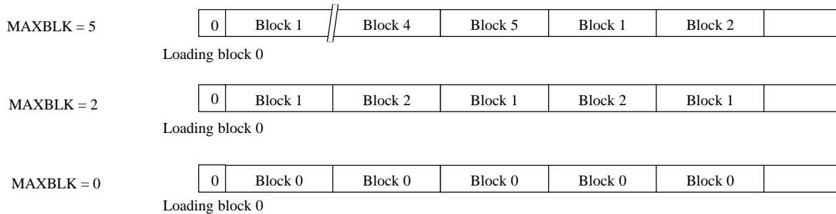
Figure 12. MAXBLK examples
