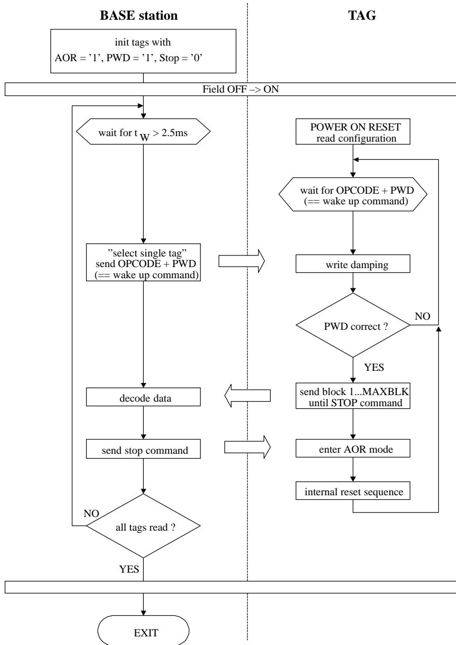
Figure 14. Anticollision procedure
