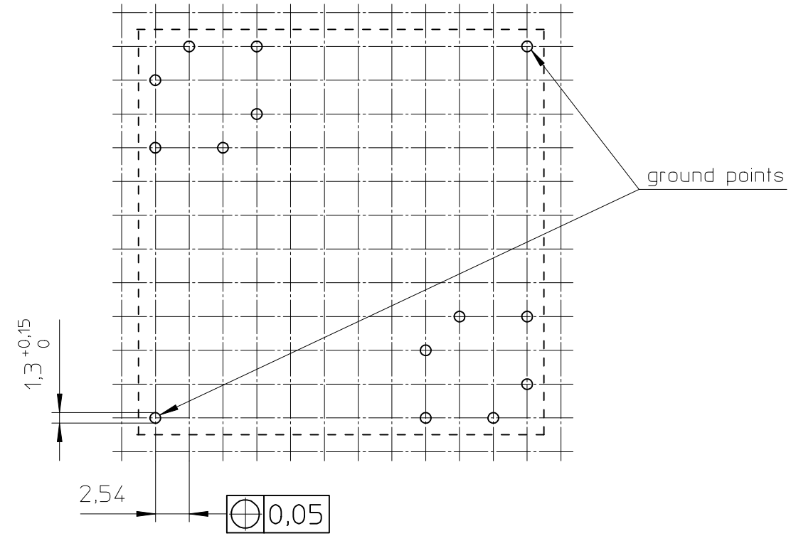
HOLE PATTERN: Space requirement 12x12 pitch
