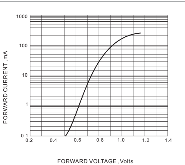
FIG. 1-TYPICAL FORWARD CHARACTERISTIC
