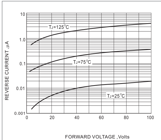
FIG. 2-TYPICAL REVERSE CHARACTERISTICS
