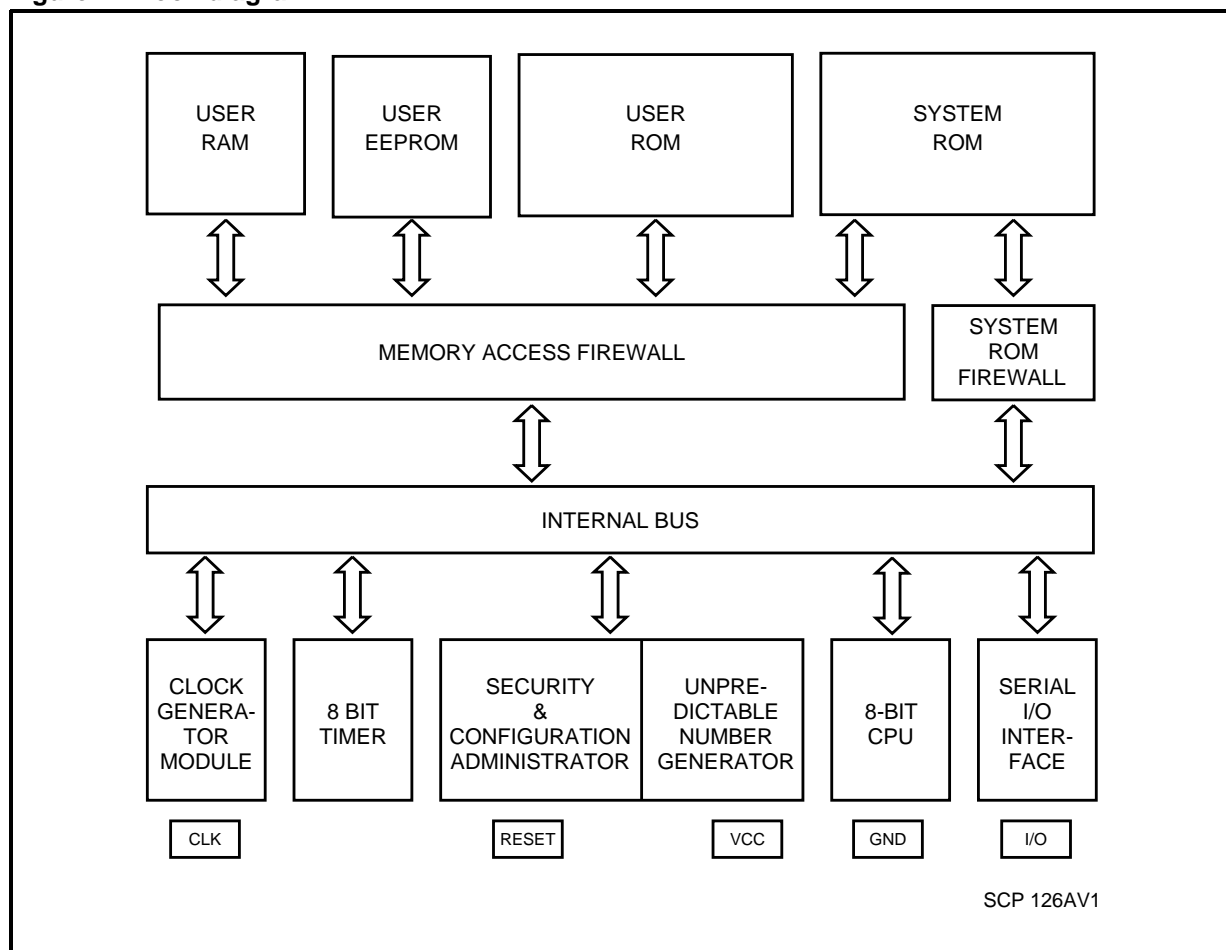
Figure 2. Block diagram
