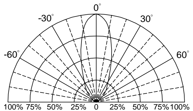
Fig.6 Directivity Radiation
